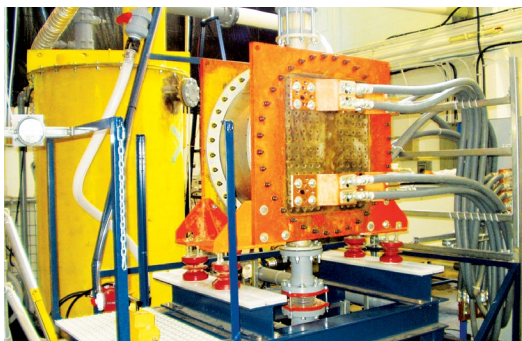
Pilot scale chlorate electrochemical cell
