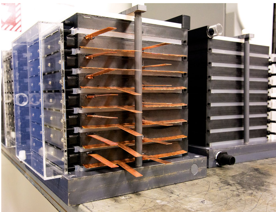
Fabricated stacks of zinc air flow cells prior to battery unit assembly
